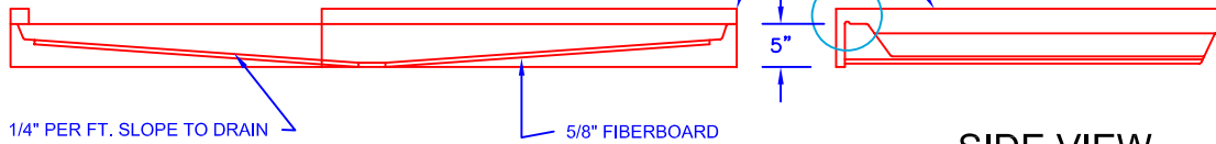
FRONT VIEW
